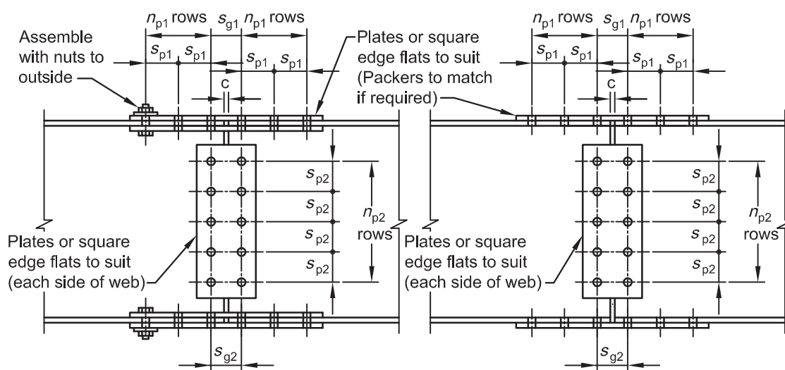
(a) Bolted moment splice in beam - Three plate flange splice - Web plate each side
