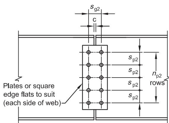
(c) Bolted shear splice in beam - Web plate each side
