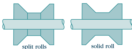
Figure 4 – Roll-former roll types
