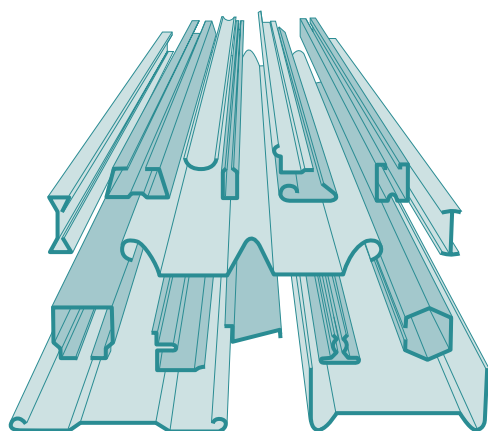
Figure 2 – Typical examples of sections produced by roll-forming
