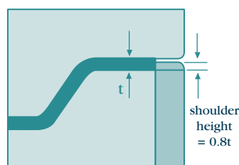
(b) Locking by a separate roll segment is a better solution
