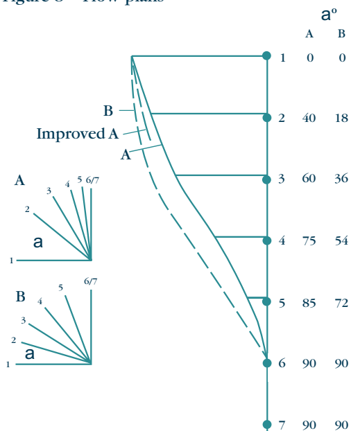
Figure 8 - Flow plans
