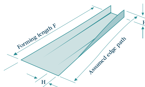
Figure 7 - Forming path
