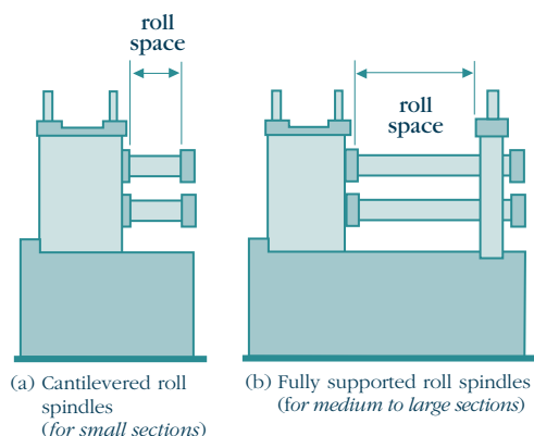
Figure 3 – Two basic roll-forming machine designs
