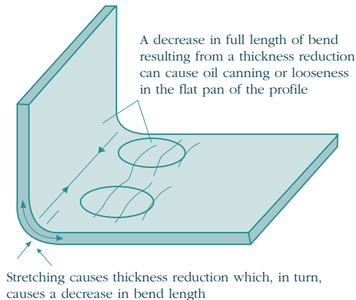
Figure 9 – Effect of transverse stretching of bends in a roll-formed profile
