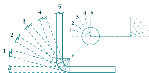
(a) Conventional forming of ductile steels
