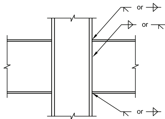
FIGURE 2 TYPICAL WELDED BEAM TO COLUMN MOMENT CONNECTION
