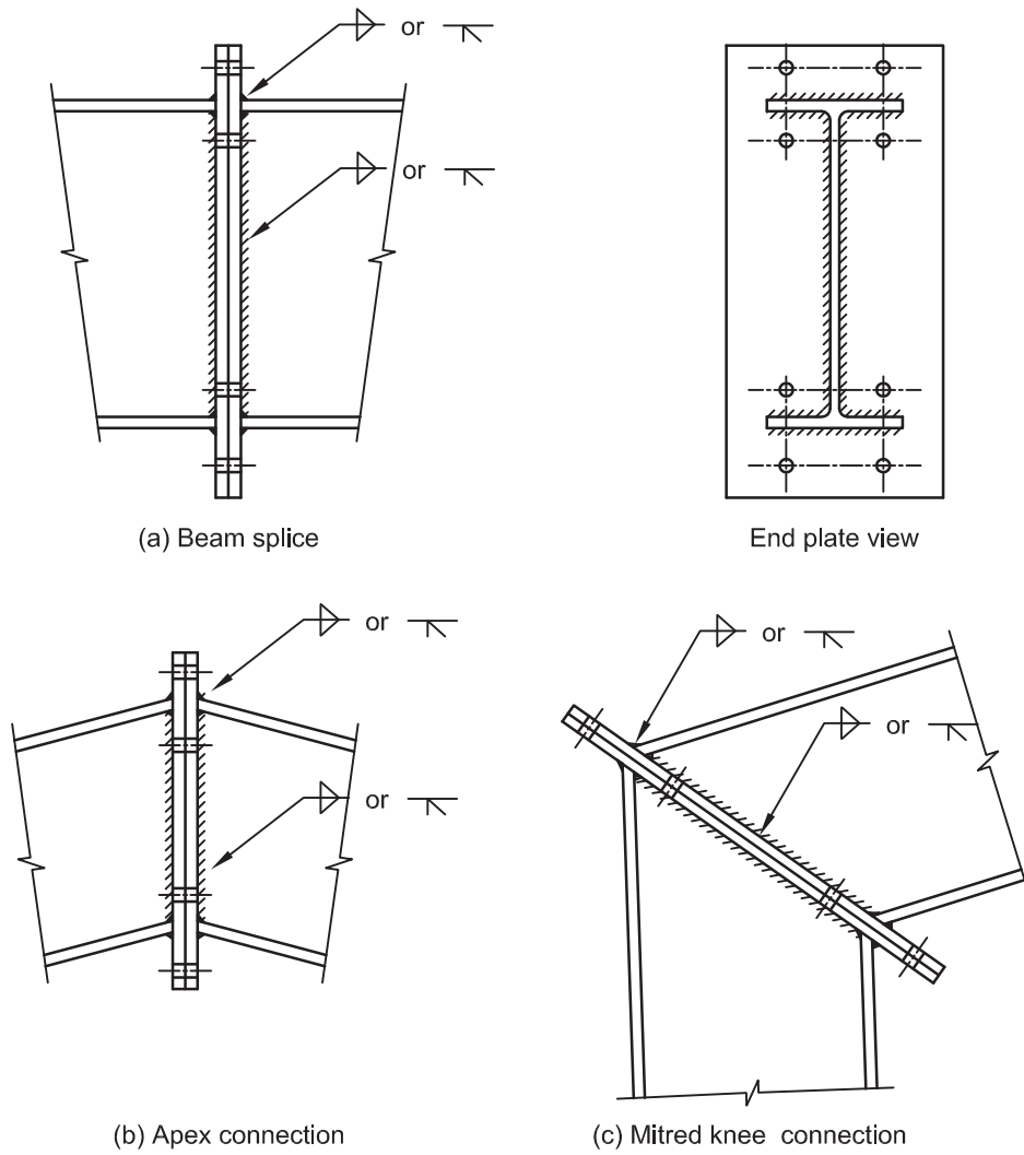
FIGURE 1 TYPICAL DETAILING FOR UNSTIFFENED VARIATIONS OF EXTENDED BOLTED MOMENT END PLATE
