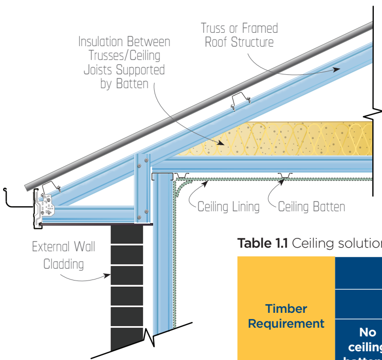
Pitched Trussed Roof, Horizontal Ceiling
